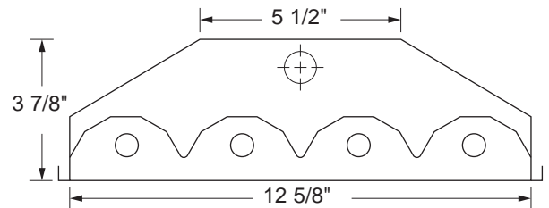
4-Lamp High Bay End View
