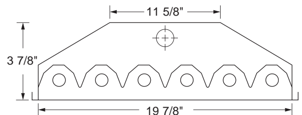
6-Lamp High Bay End View
